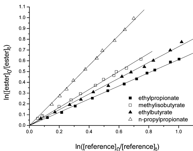
Figure 2. Relative rate data for the Cl reactions with the investigated esters.
